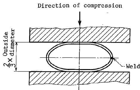
Fig. 2. Flattening Test
