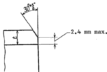
Fig. 1. Shape of Bevel End
